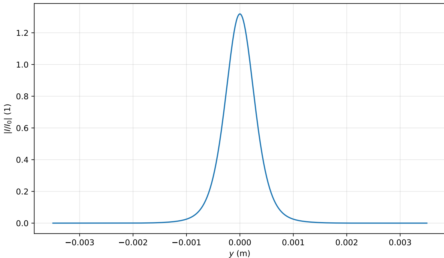
Intensity profile I(x=0, y, z=1.990)/I_0 , P_{in}=0.8P_{cr} , artificial time
